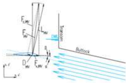
Fig.3. Forces acting on the hull vane
