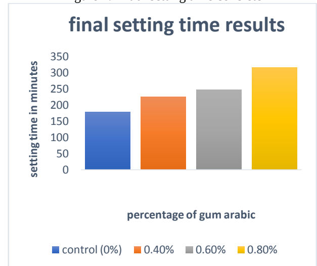
Figure 3. final setting time concrete
