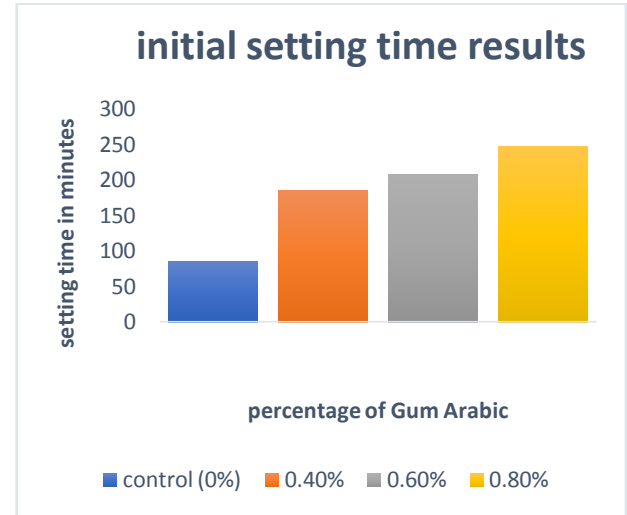
Figure 2. initial setting time concrete
