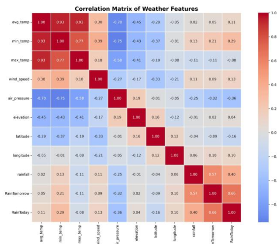
Fig. 2. Pearson Correlation Matrix Heatmap of all meteorological weather features.
