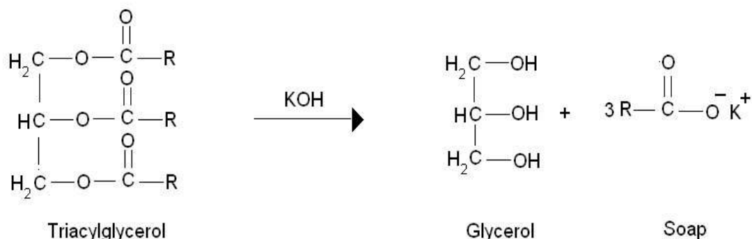
Figure 4; Soap formation from saponification reaction
