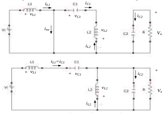
Fig. 2. Circuit with switch ON and OFF states
