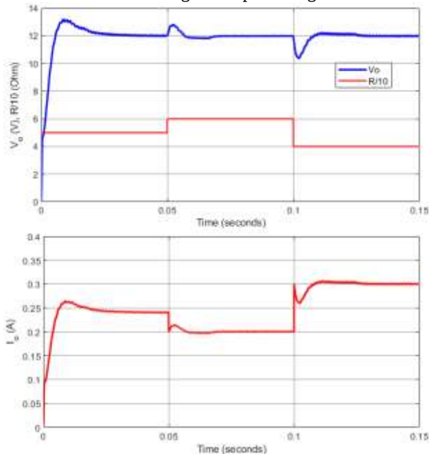
Fig. 11. Output voltage waveforms with changes in load
