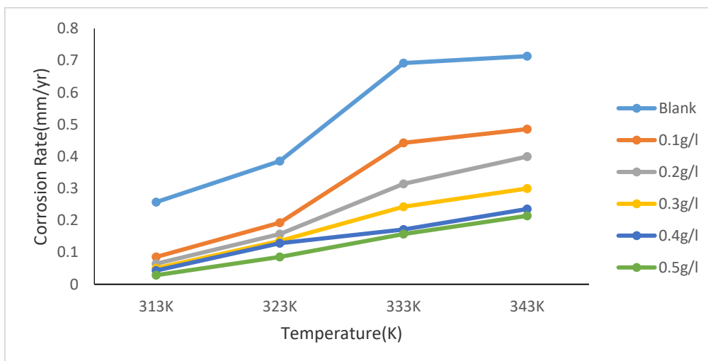
Figure 6: Corrosion Rate against Temperature of Hyptis Suaveolens Extract at Elevated Temperature
