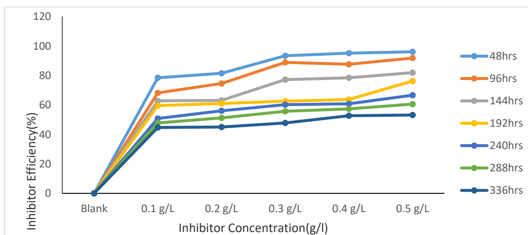
Figure 5: Inhibition Efficiency against blends of Hyptis suaveolens extract in 1M H 2 SO 4 and nanoparticles obtained from the barks of Ficusthonningii inhibitor concentration at room temperature (30±2)
