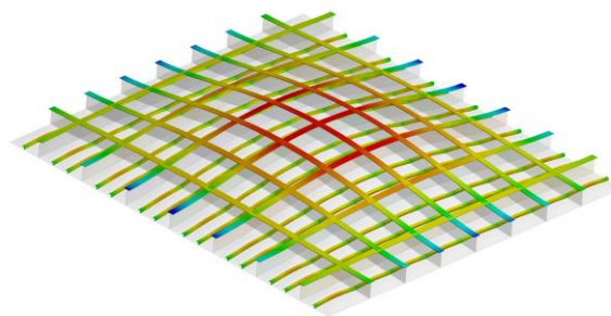
Fig. 9. Stress at Flanges
