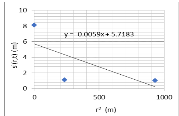
Figure.19. graph with Straight-line of s'(r,t) and r^2 and estimate values of slope and intercept. Data from (Dessurealt, Aquifer of Saint-Henri de Taillon, Quebec, Canada 1975. P 72-76).
