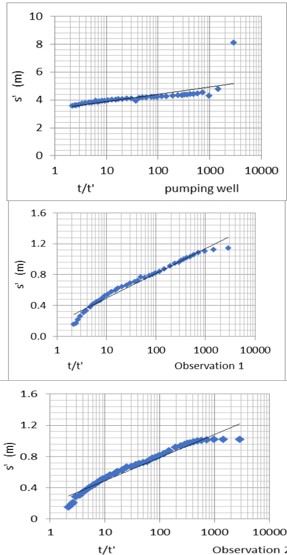
Figure.13. (a.b.c) graph with Straight-line of drawdown and t/t' and estimate values of slope for each well. Data from (Dessurealt, Aquifer of Saint-Henri de Taillon, Quebec, Canada 1975. P 72-76).
