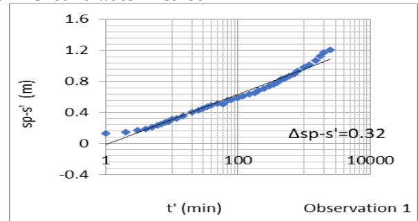
Figure.13. (a.b.c) graph with Straight-line of drawdown and t/t' and estimate values of slope for each well. Data from (Dessurealt, Aquifer of Saint-Henri de Taillon, Quebec, Canada 1975. P 72-76).
