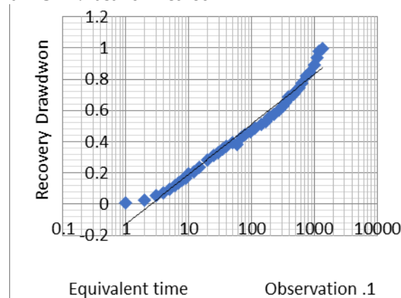
Figure.22. (a) Semi-log graph with Straight-line of recovery drawdown and equivalent time. And estimate values of slope and intercept for each well. Data from (Dessurealt, Aquifer of Saint-Henri de Taillon, Quebec, Canada 1975. P 72-76).
