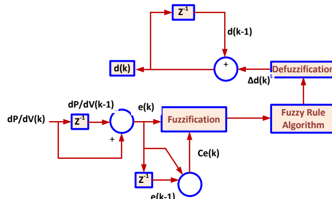
Fig. 7 Structure of Fuzzy Logic Controller
