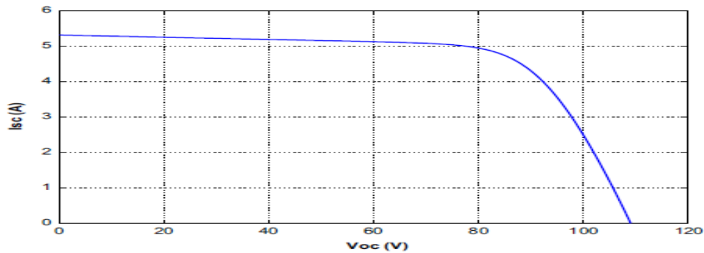
Fig. 4. I-V Characteristics of a typical PV array
