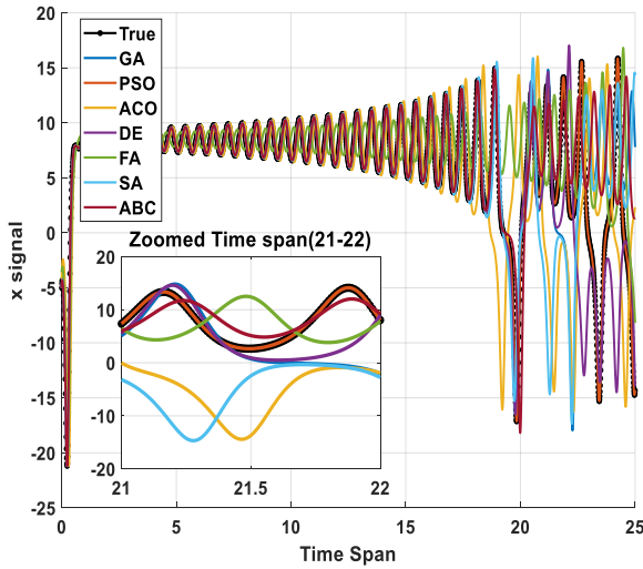
Fig. 7. Reconstruction of the x-component of the Lorenz signal using estimated initial conditions from various optimization algorithms, with a detailed view of the time interval between 21 and 22.
