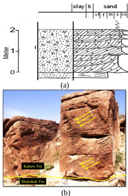
Fig. 2. (a,b) Medium to very coarse -grained planar and trough cross - bedding sandstone unconformably overlie the Shakshuk Formation, in addition to clarifying my drawing for part (FA1) bedding (Ganawan section).
