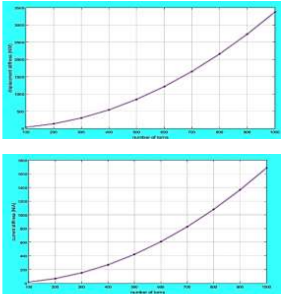
Fig.8.The displacement stiffness and current stiffness vs number of turns
