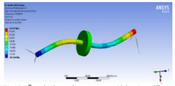
Fig.15. 4 th mode shape of rotor system with bearing stiffness at natural frequency = 718.68Hz
