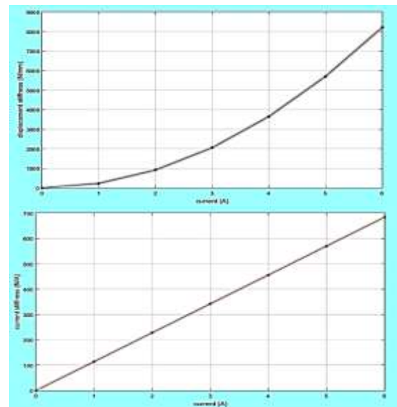
Fig.10.The displacement stiffness and current stiffness vs current
