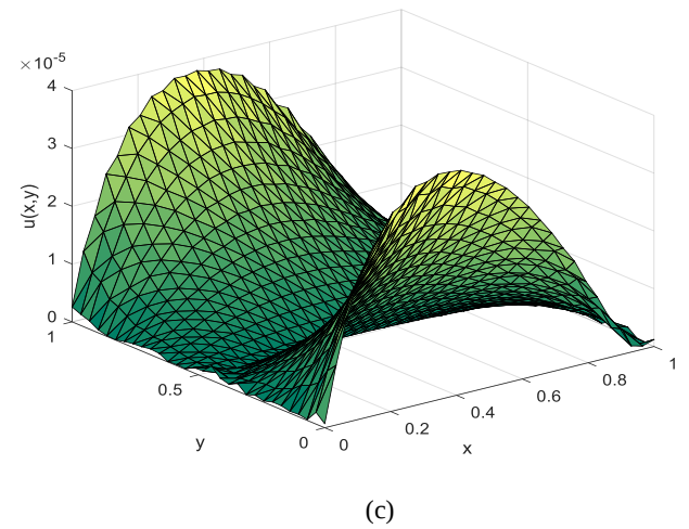
Figure 6: Numerical Solution of Example 3.2 on Equally Spaced Data Points using (a) MQ (b) GMQ( \beta = 1.03 ) and (c) GMQ( \beta = 1.99 )
