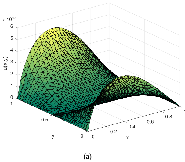
Figure 6: Numerical Solution of Example 3.2 on Equally Spaced Data Points using (a) MQ (b) GMQ( \beta = 1.03 ) and (c) GMQ( \beta = 1.99 )
