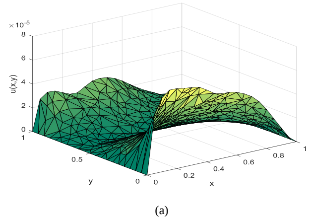
Figure 6: Numerical Solution of Example 3.2 on Equally Spaced Data Points using (a) MQ (b) GMQ( \beta = 1.03 ) and (c) GMQ( \beta = 1.99 )
