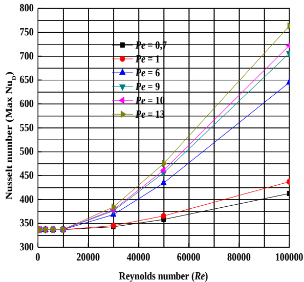
Fig.7. Variation of Nusselt number Nu_D versus Reynolds number for various values of Pe
