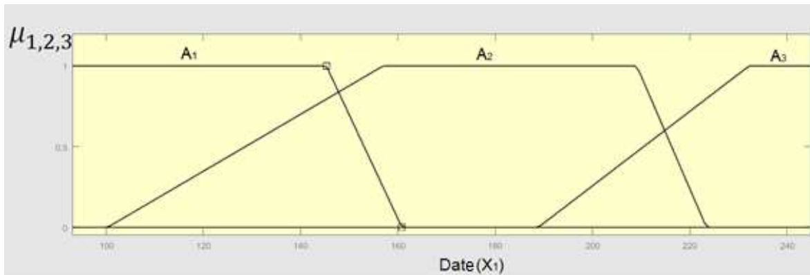
Figure 1 - membership functions.
