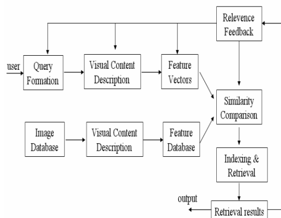
Figure1. Block Diagram of CBIR System
