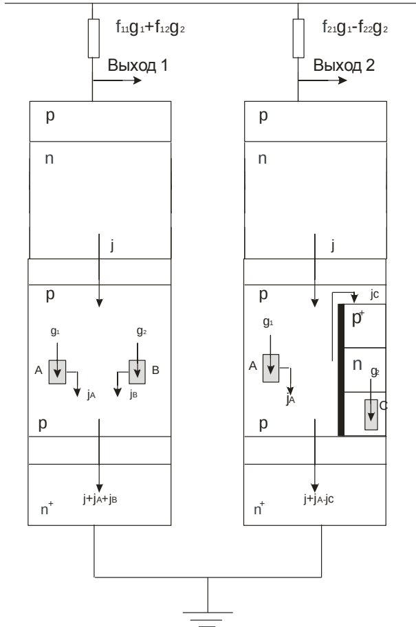
Fig. 2. A model structure of s/c device of division signal-noise.
