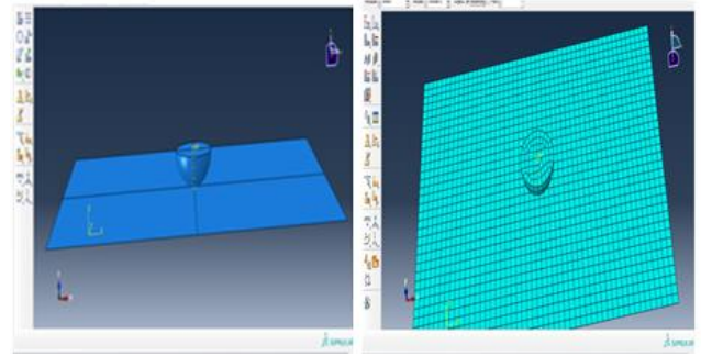
Fig. 3. Finite element model of composite laminate before impact loading.
