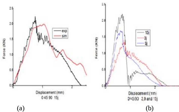
Fig.13. F-D curve of G16
