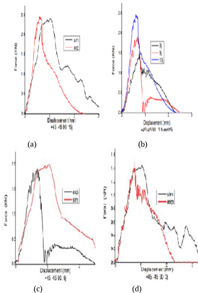
Fig.12. F-D curve of G26
