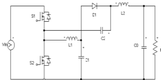
Fig. 2. Circuit Diagram of KY Buck-Boost Converter
