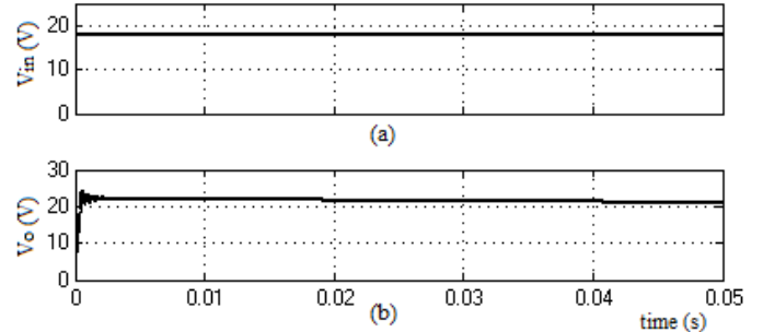
Fig. 11. Simulink result (a) Input Voltage( V_{in} ) and (b) Output Voltage( V_o )
