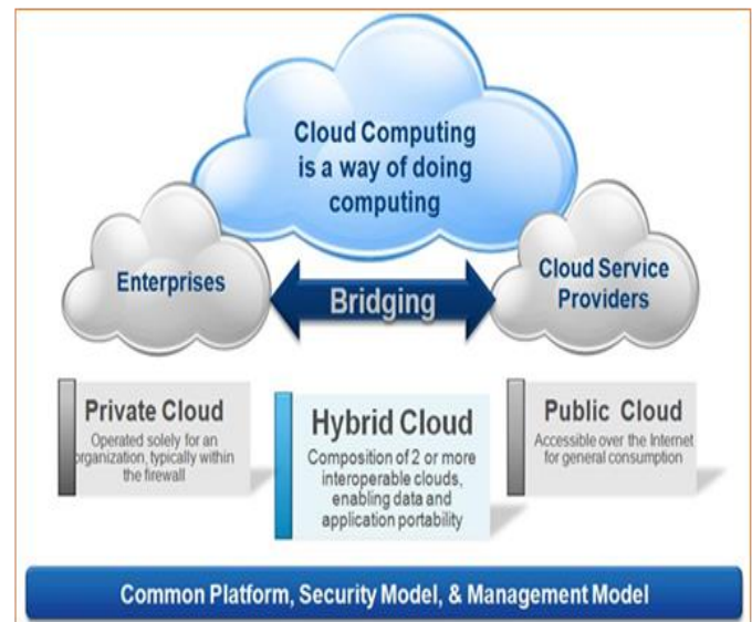
Fig3. Cloud Model [16]
