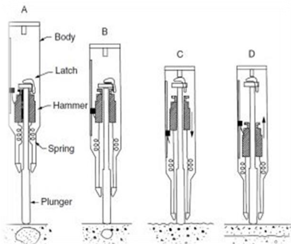
Figure 2: Schematic diagram of Schmidt rebound hammer procedure [9]
