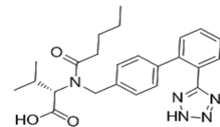
Fig. 2: Structure of valsartan
