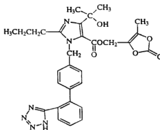
Figure 1: Olmesartan Medoxomil
