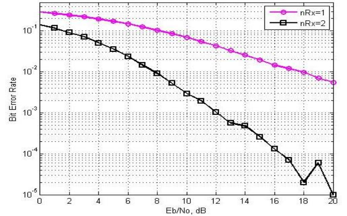
Fig.5 BER for QPSK using EGC
