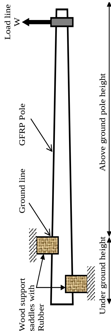
Fig. 2. Specified methods for testing FRP poles
