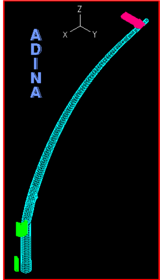
Fig. 3. Failure mode
