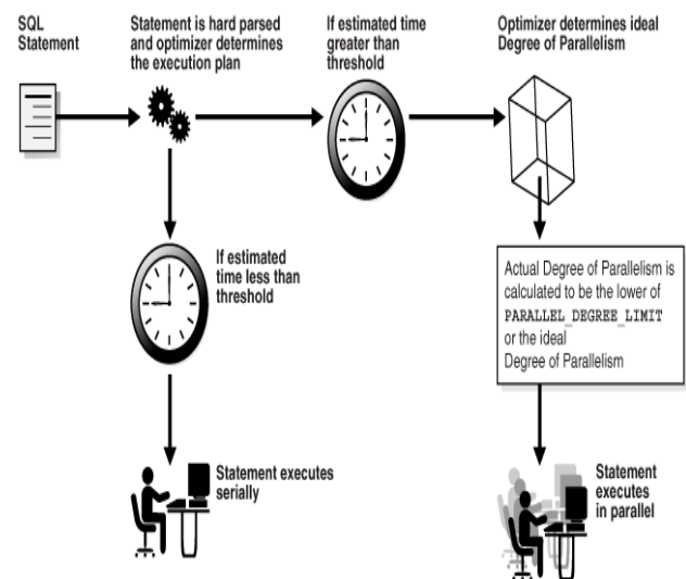
Fig1.optimizer calculation: Serial or Parallel [11]
