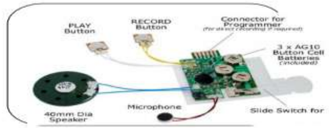
Fig6.WORKING OF APR9600
