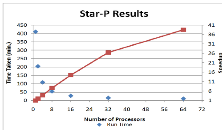
Fig. 8. Star-P Results
