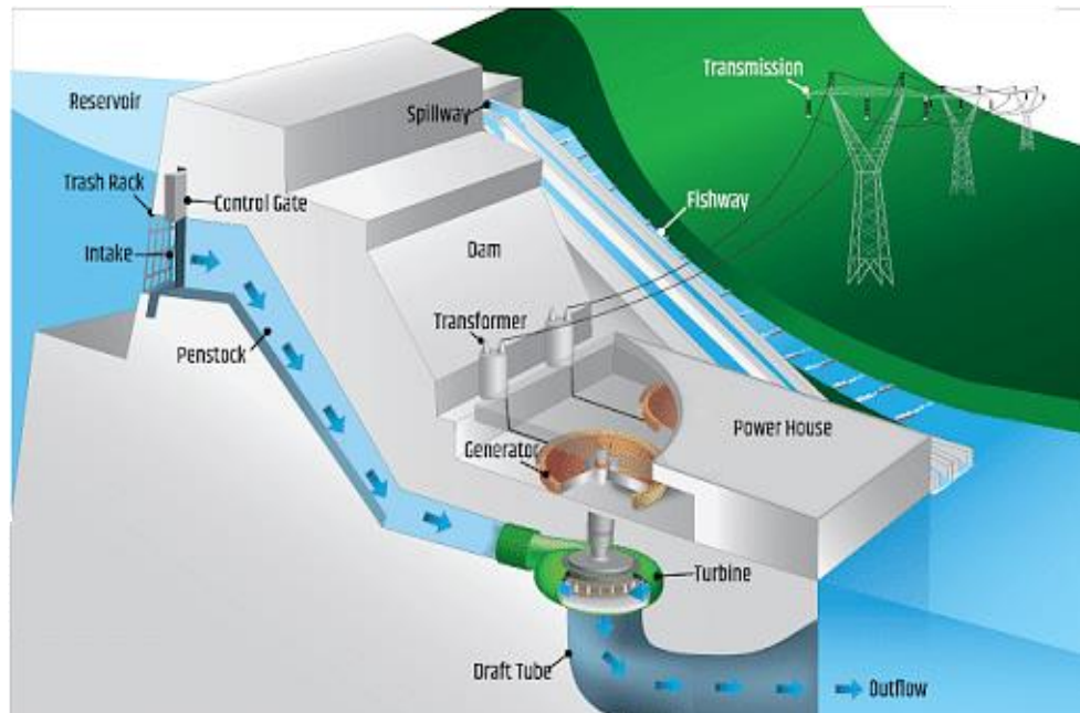
Figure 4: Hydropower system (Bayar and Gavriltea, 2019; Maji et al., 2019).
