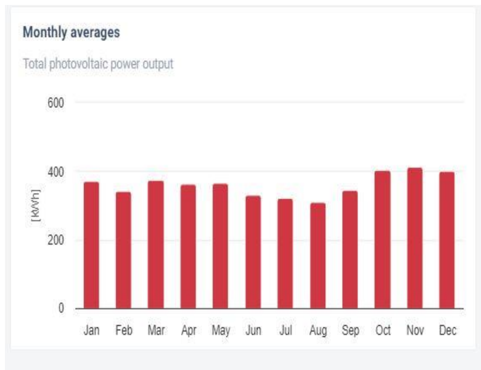
Figure 11: Monthly Average Photovoltaic power Output
