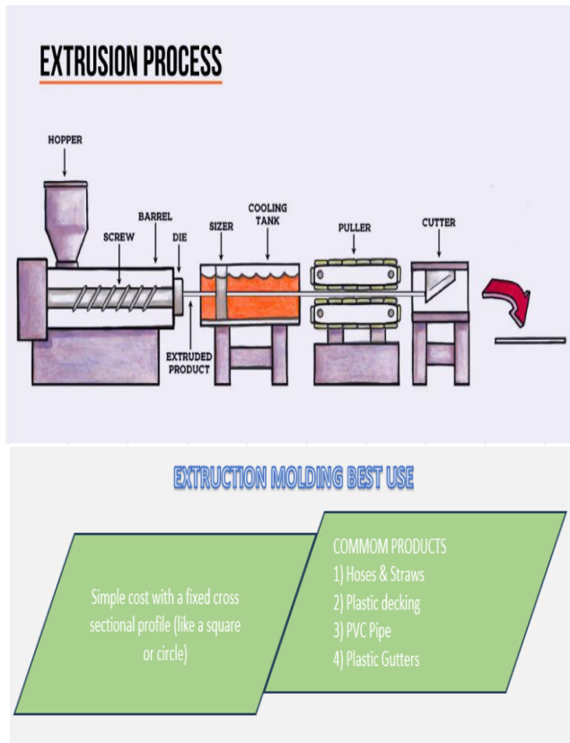
Extrusion Molding
