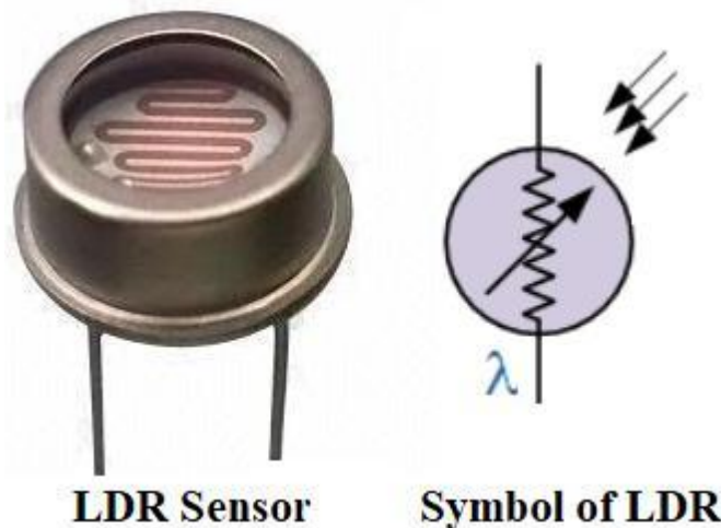
Fig. 3. LDR Sensor
