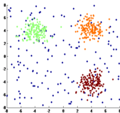
Fig 3: Unsupervised learning
