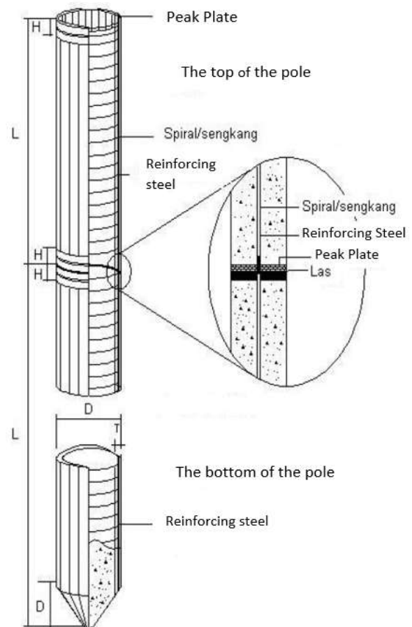
Fig. 1 Construction of Round Pile Connections with Welding
