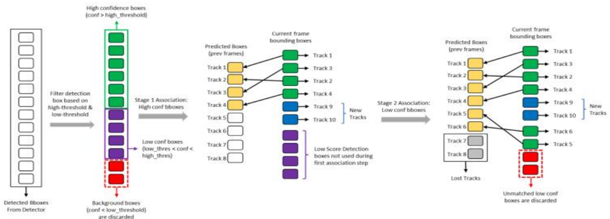
Fig. 2. ByteTrack Model Architecture [12]
