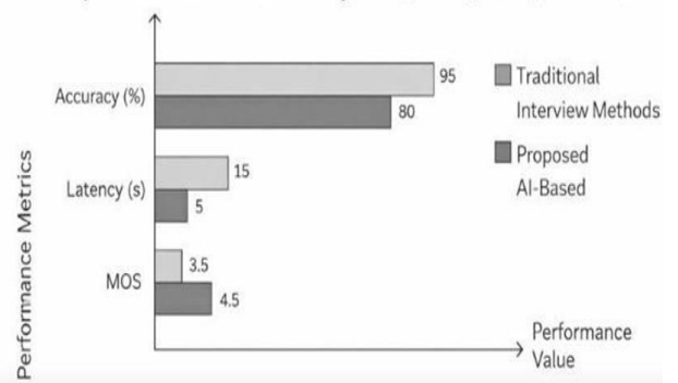
Fig 5. Performance Comparison of Traditional and Proposed AI Based Interview System
