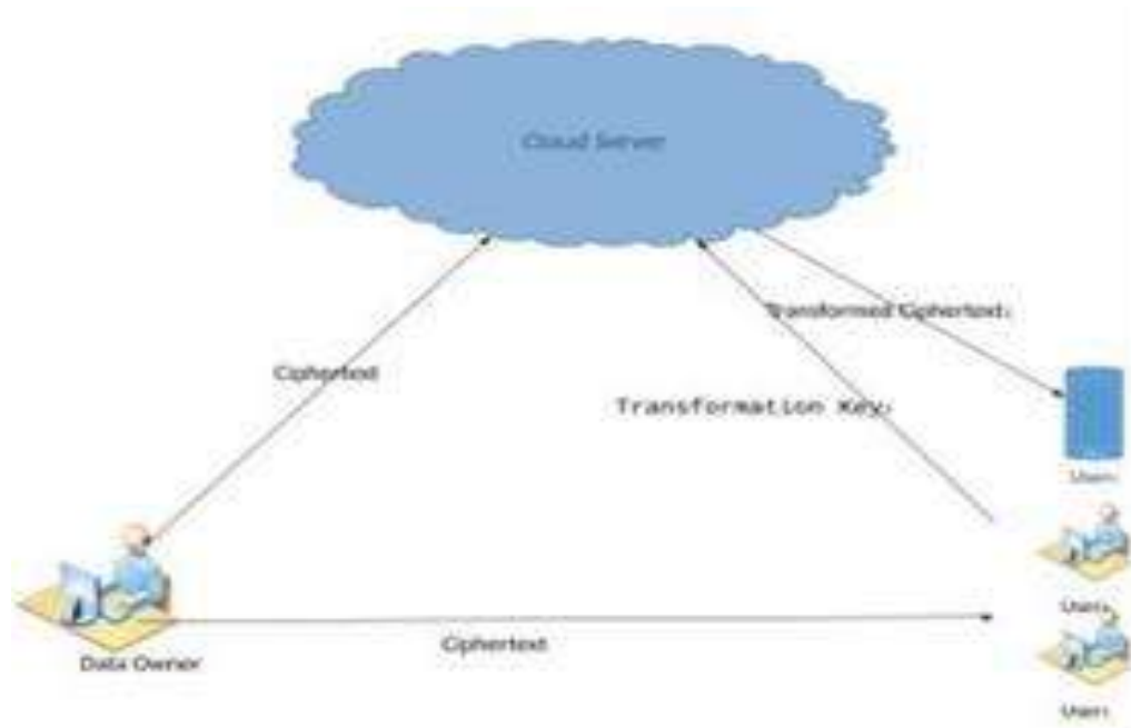
Figure 1. Architecture for ABE-OD
