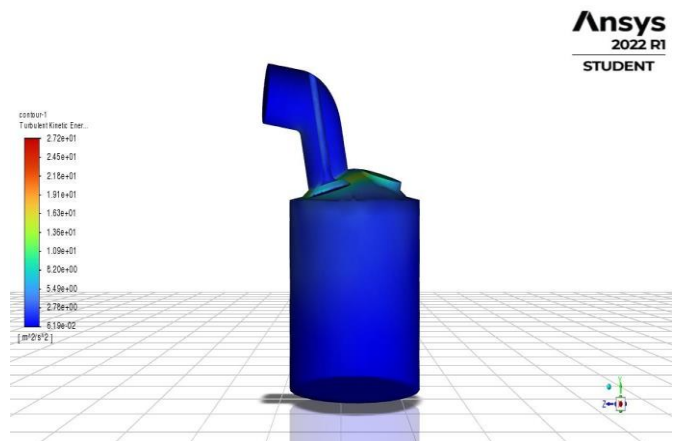
Figure.15 Turbulence Energy Contour in Grooved Cylinder Head
