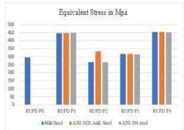
Fig.15.Graph showing Equivalent Stress (in Mpa).
