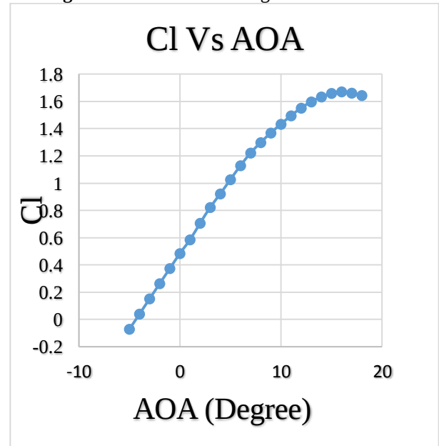
Figure2: Coefficient of lift w.r.t AOA
