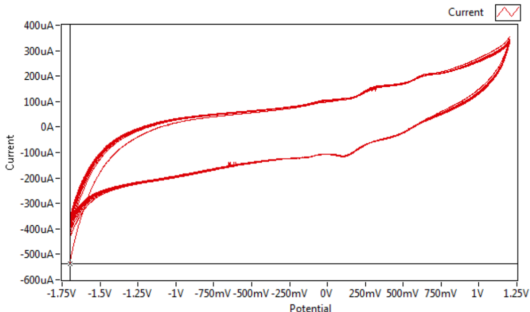
Fig. 11: Cyclic voltammogram of 0.38 mM PAR at ten times on the modified electrode (fMWCNT/GCE) versus Ag/AgCl as a reference electrode
