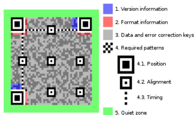
Fig. 1. QR Code Structure
