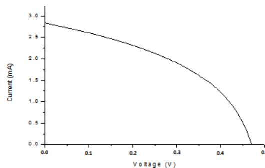
Figure 2: J-V curve for the device DG6
