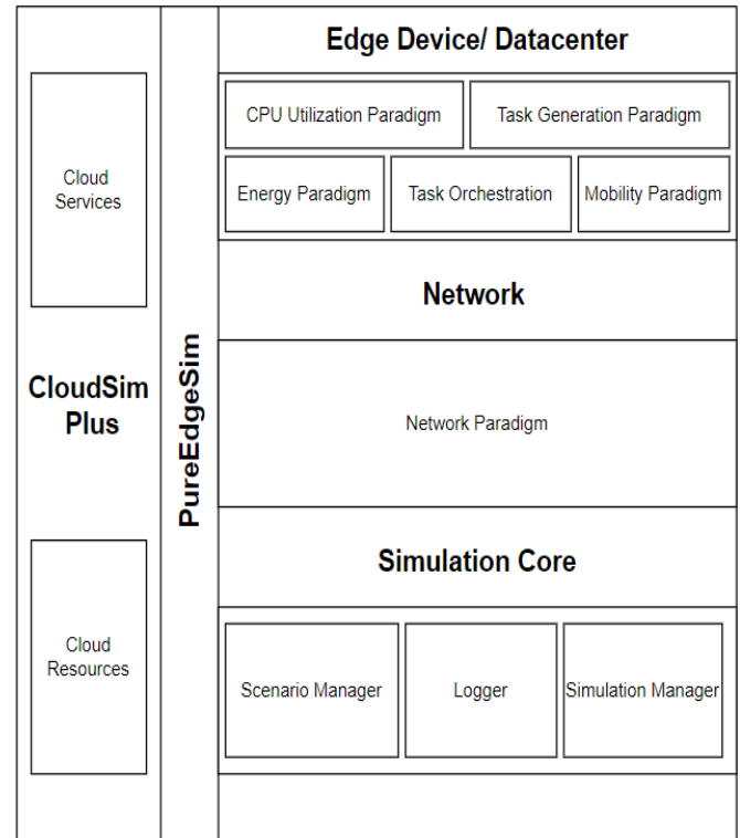
Figure 1. PureEdgeSim Architecture
