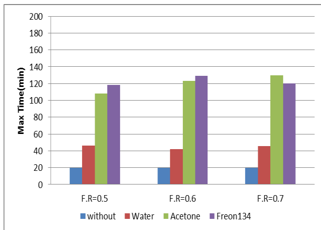
Figure 7:relationship between maximam heating time for the working fluids and filling ratios for power supply 200 W
