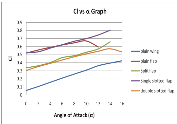
Fig.4. C_l vs \alpha Graph of NACA 2412 Aerofoil with different types of flaps
