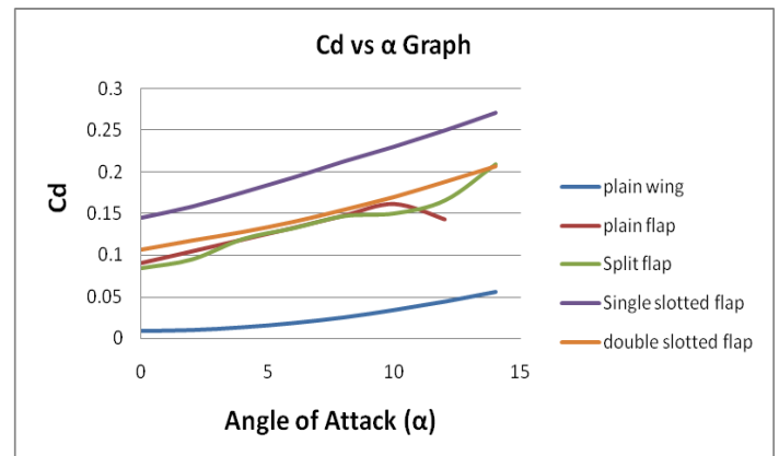
Fig.5. C_d vs \alpha Graph of NACA 2412 Aerofoil with different types of flaps
