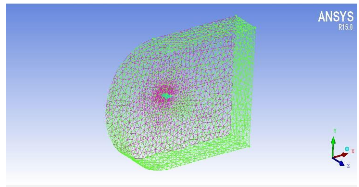
Fig.2. Surface meshing of the domain containing the plain wing with NACA 2412 aerofoil profile.
