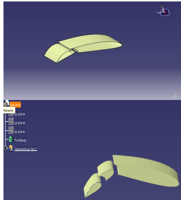
FIG.1. CATIA model of Plain wing, Plain flap, Split flap, Single Slotted flap and Double Slotted flap at fixed 10° angle of attack
