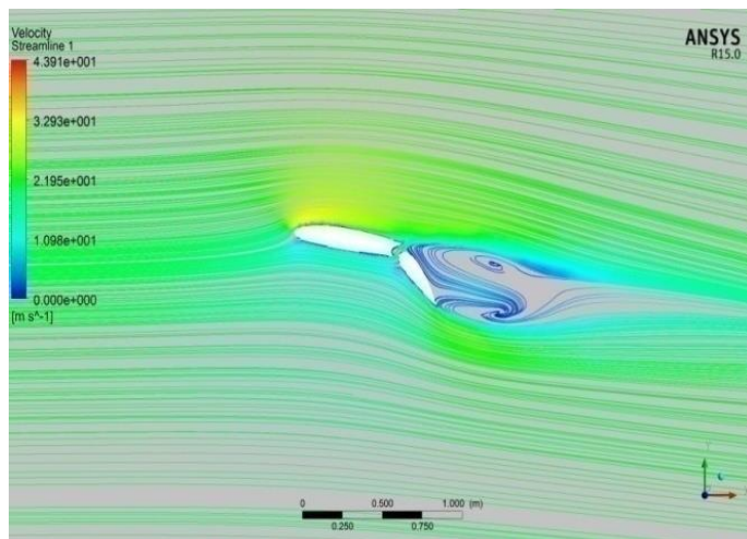
Fig.7. Streamline of velocity magnitude on NACA 2412 aerofoil with Single slotted Flap at 10°, also showing turbulent flow at trailing edge.
