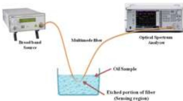
Fig. 2: Experimental arrangement
