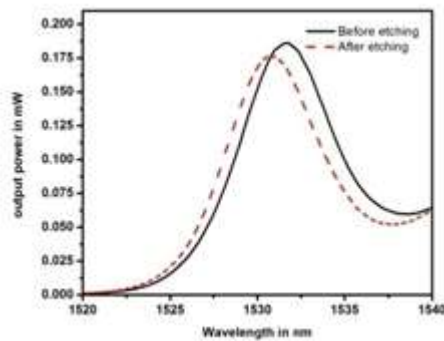
Fig.3: Output power versus Wavelength comparison of etching
