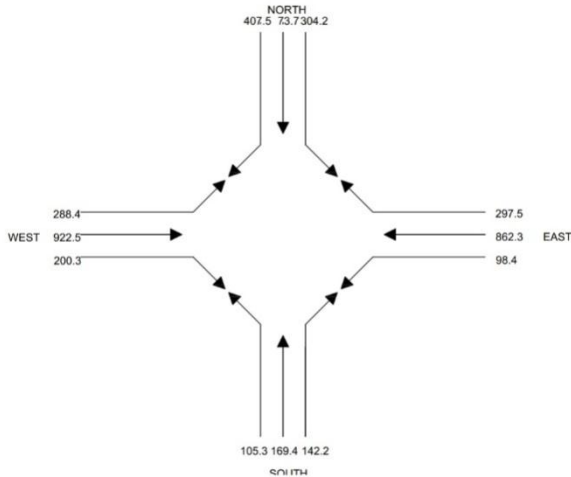
Fig No.7.2: Traffic approaching from each leg to roundabout in PCU/hr.
