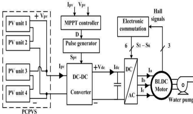
Fig. 1. Schematic of conventional DC-DC converter based PV water pumping system
