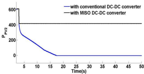
Fig. 5. Variation in PV unit 2 power with change in irradiation
