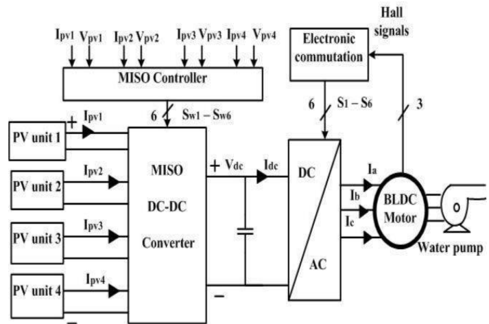
Fig. 2. Schematic of proposed MISO DC-DC converter based PV water pumping
