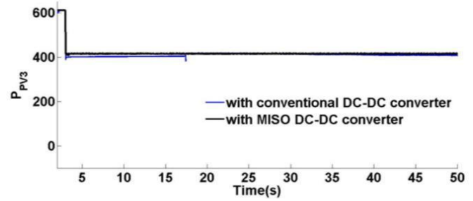
Fig. 6. Variation in PV unit 3 power with change in irradiation
