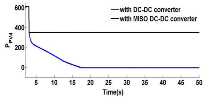
Fig. 7. Variation in PV unit 4 power with change in irradiation
