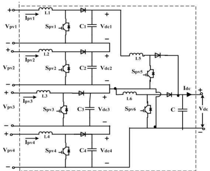
Fig. 3. Configuration of proposed MISO DC-DC converter
