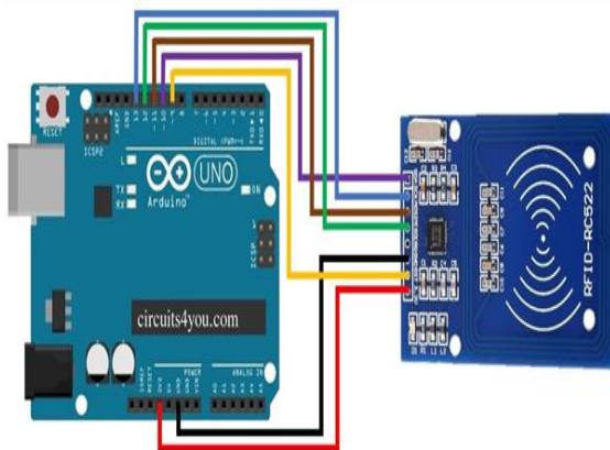
Figure (e) interface between RFID Reader and Arduino
