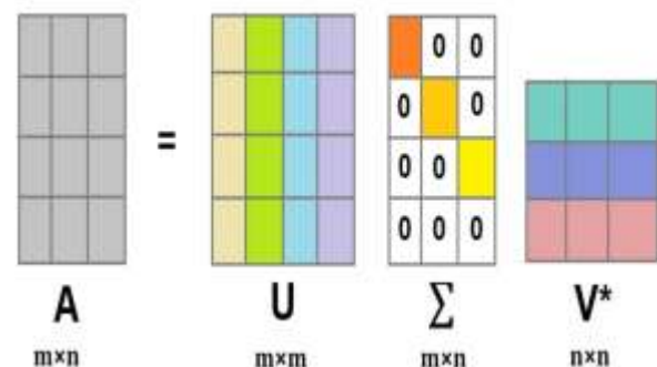
Figure 1: Singular Value Decomposition Matrix.
