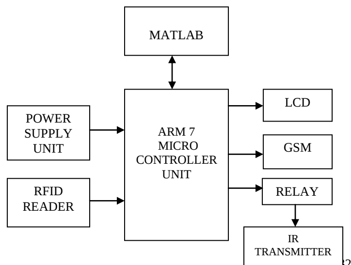
Fig.1. Block Diagram
